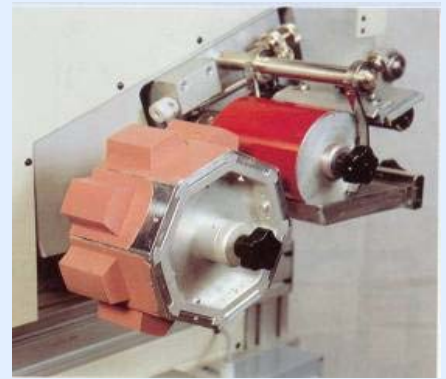
Rotary pad printer
