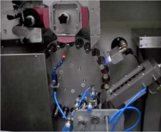
Rotary Pad Printing System with Flame Treater, Part Loader and Unloader
