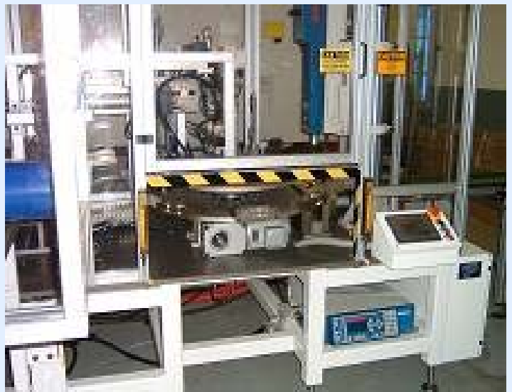
Rotary Index Table with Ultrasonic welding station
