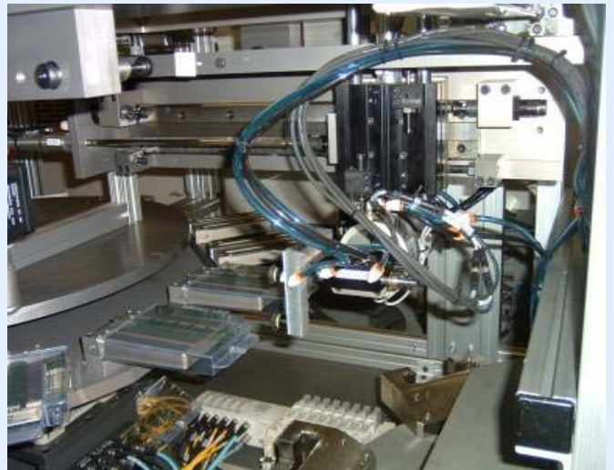
Part transfer module with X-Y-Z-R motion
