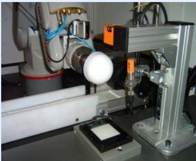
Robot Inspection System
